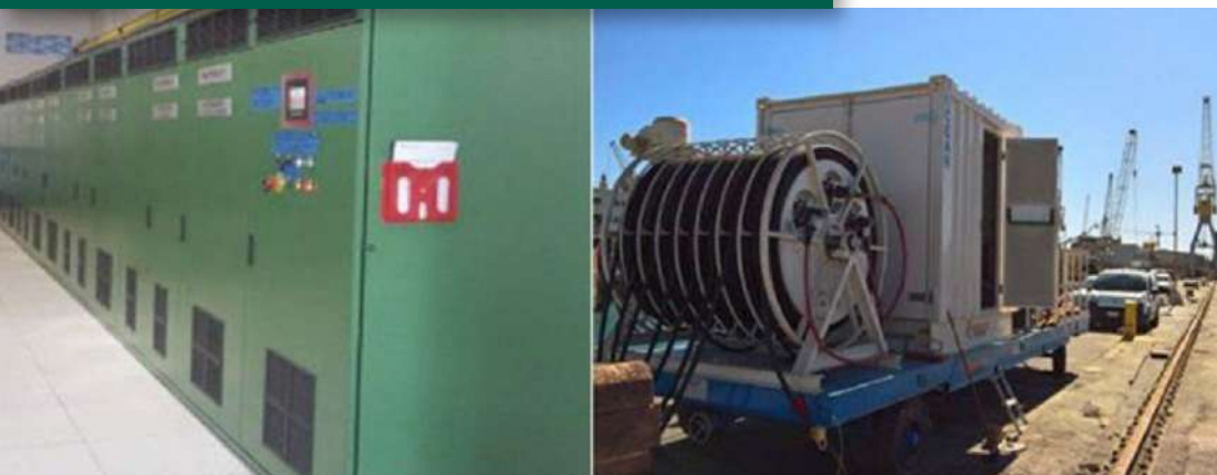
Cold ironing facilities in the Genova Pra' Terminal
