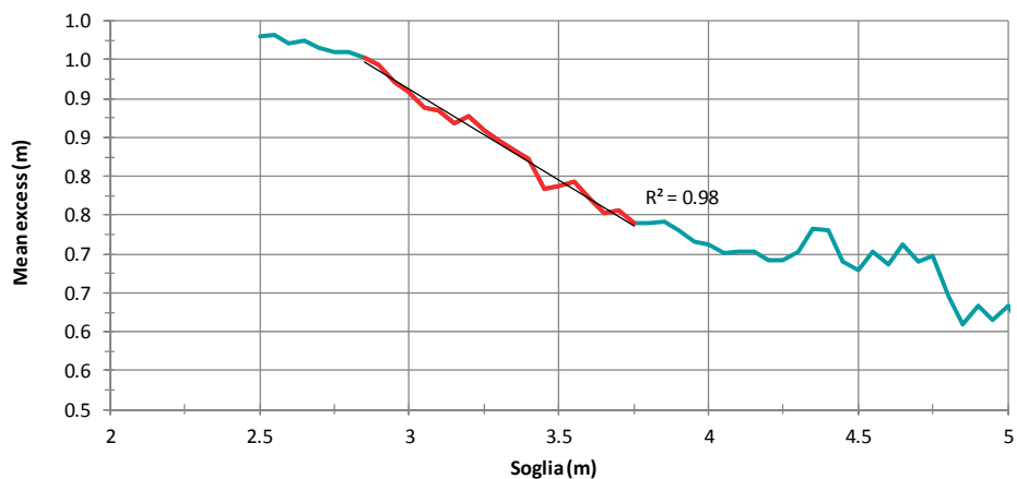
FIGURA 8-5 - MEAN RESIDUAL LIFE PLOT - OVERALL: 90 - 270°N
